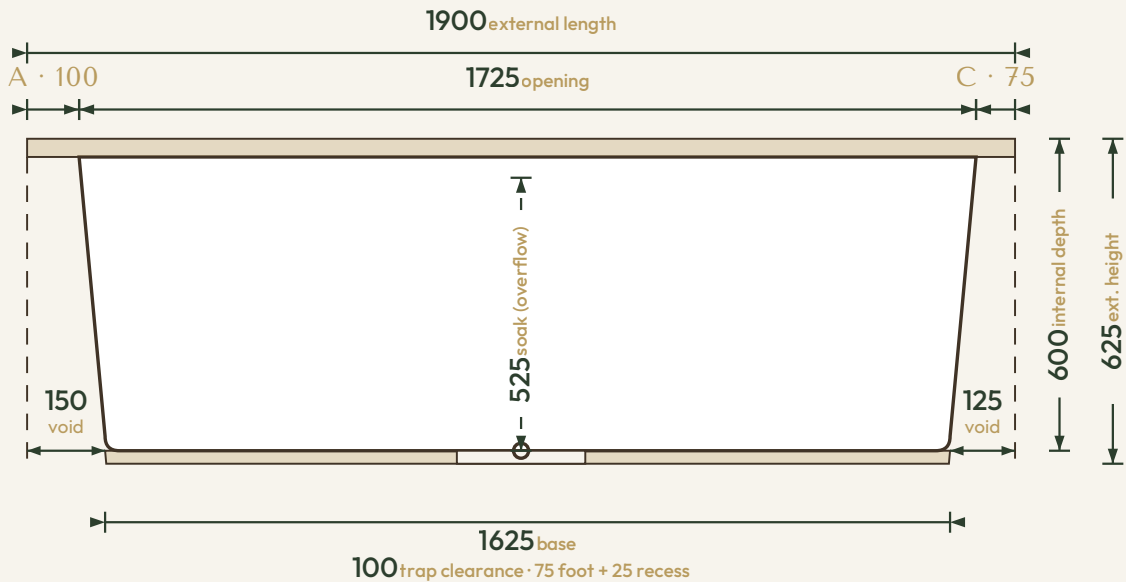
SIDE PROFILE
