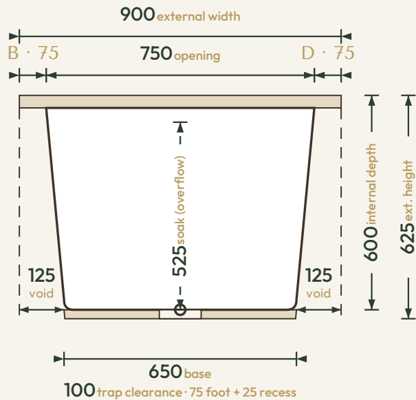
END PROFILE
